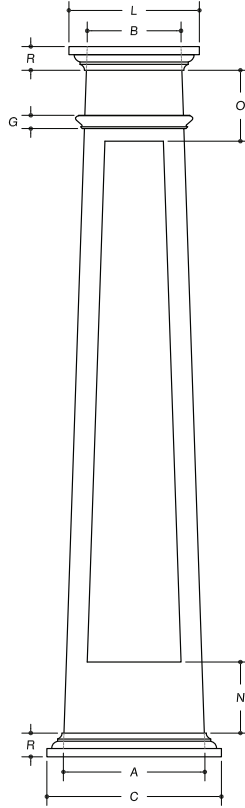
Fig. 3 Craftsman with Traditional Cap & Base
