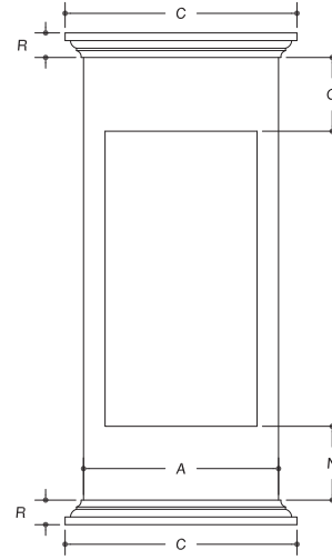
Fig. 4 Pedestal with Traditional Cap & Base
